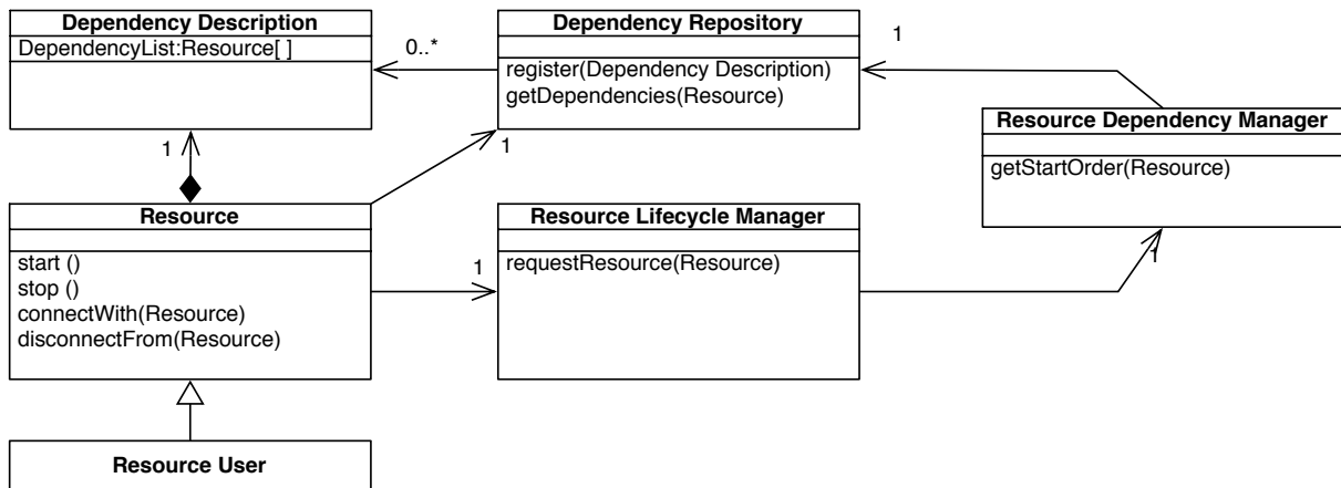
Fig. 2. Class diagram of the Resource Dependency Manager pattern.
