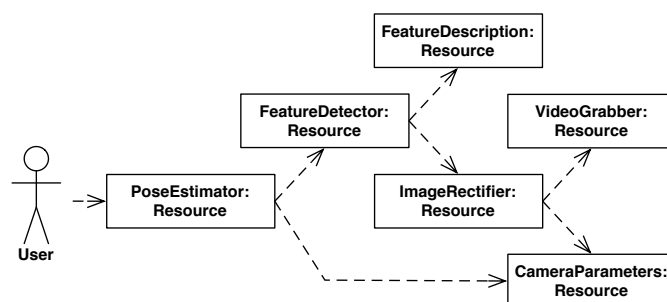
Fig. 1. A user acquires a resource which transitively uses other resources it depends on.
